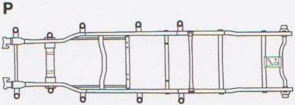
P D UNDERBODY VIEW
